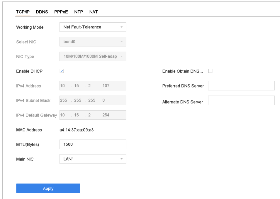
Figure 3-5 Network Settings
