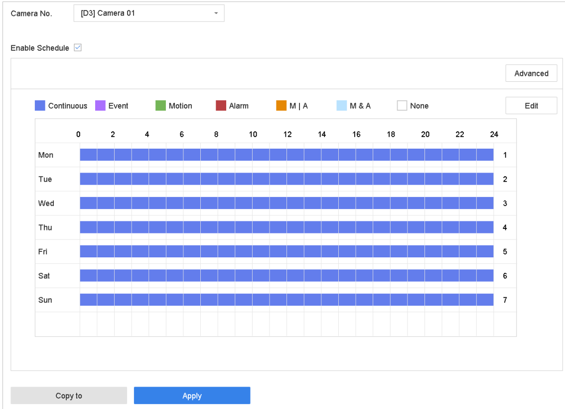
Figure 3-8 Record Schedule
